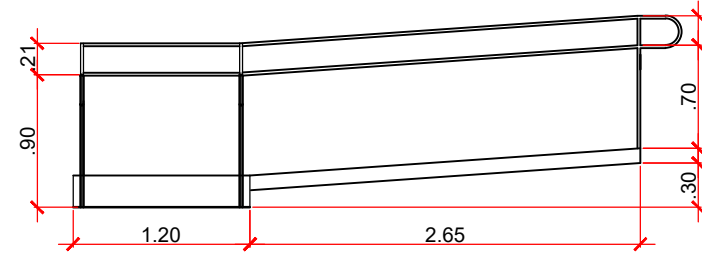
VISTA FRONTAL
